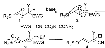
Scheme 1. Epoxysilane rearrangement.
